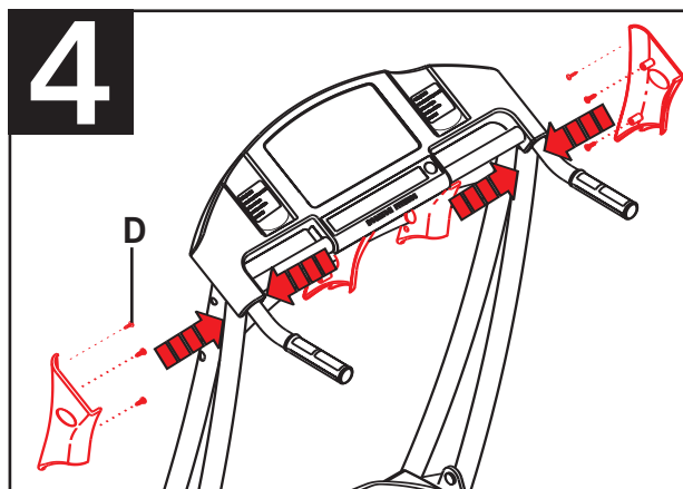
STEP 4: ATTACH LEFT & RIGHT CONSOLE MAST COVERS/BOOTS.
