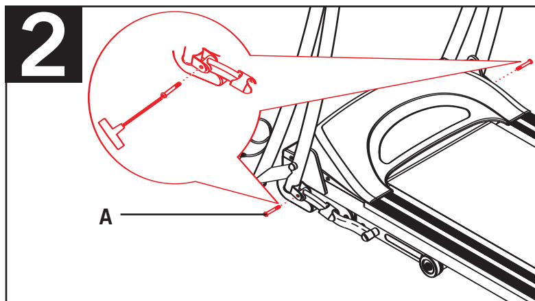
STEP 2: SECURE AND TIGHTEN ALL BOLTS.
