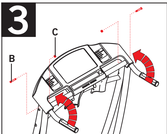
STEP 3: ATTACH CONSOLE CABLE AND LOCK CON- SOLE INTO PLACE. SECURE AND TIGHT- EN ALL BOLTS. Note: Do not pinch the wires.
