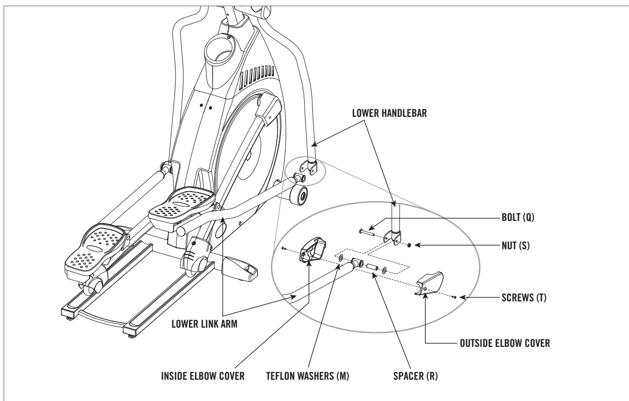
SPACER (R) 44 mm axis Qty: 2
